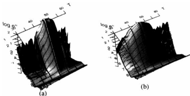
FIGURE 7. Dielectric absorption of CDMix2 in a 25\ \mu\text{m} cell. Measuring field: 20\ \text{mV}/\mu\text{m} . (a) heating at 1^\circ\text{C}/\text{min} ; (b) cooling at 1^\circ\text{C}/\text{min} .
