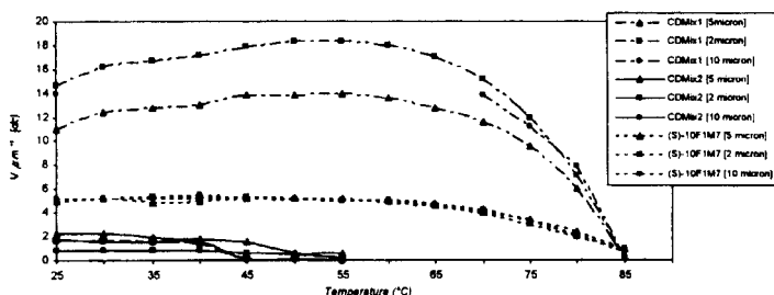
FIGURE 2. DC “after-threshold” voltages for CDMix1, CDMix2 and (S)-10F1M7 ( \text{V}\mu\text{m}^{-1} ). The measurements were taken from the point at which the spontaneous polarisation is observed on cooling from the \text{SmA}^* phase.
