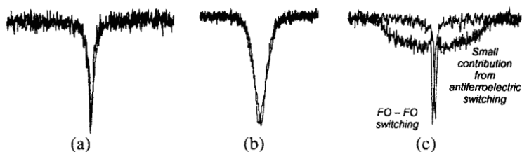
FIGURE 4. Switching behaviour of CDMix2. (a) 2 \mu\text{m} , 5 mHz (36 V pp ), (b) 5 \mu\text{m} , 5 mHz (21 V pp ), 10 \mu\text{m} , 5 mHz (41 V pp )
