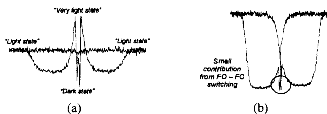
FIGURE 3. Switching behaviour in CDMix1. (a) 2 \mu\text{m} , 5 mHz (150V pp ), (b) 5 \mu\text{m} , 5 mHz (85V pp )
